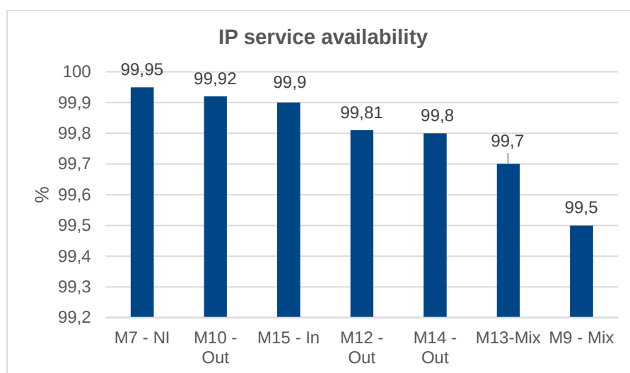
Figure 11: Average value of the achievable IP service availability during peak-time in a mobile network with fibre roll-out up to the base station and the best LTE Advanced technology used in this network
