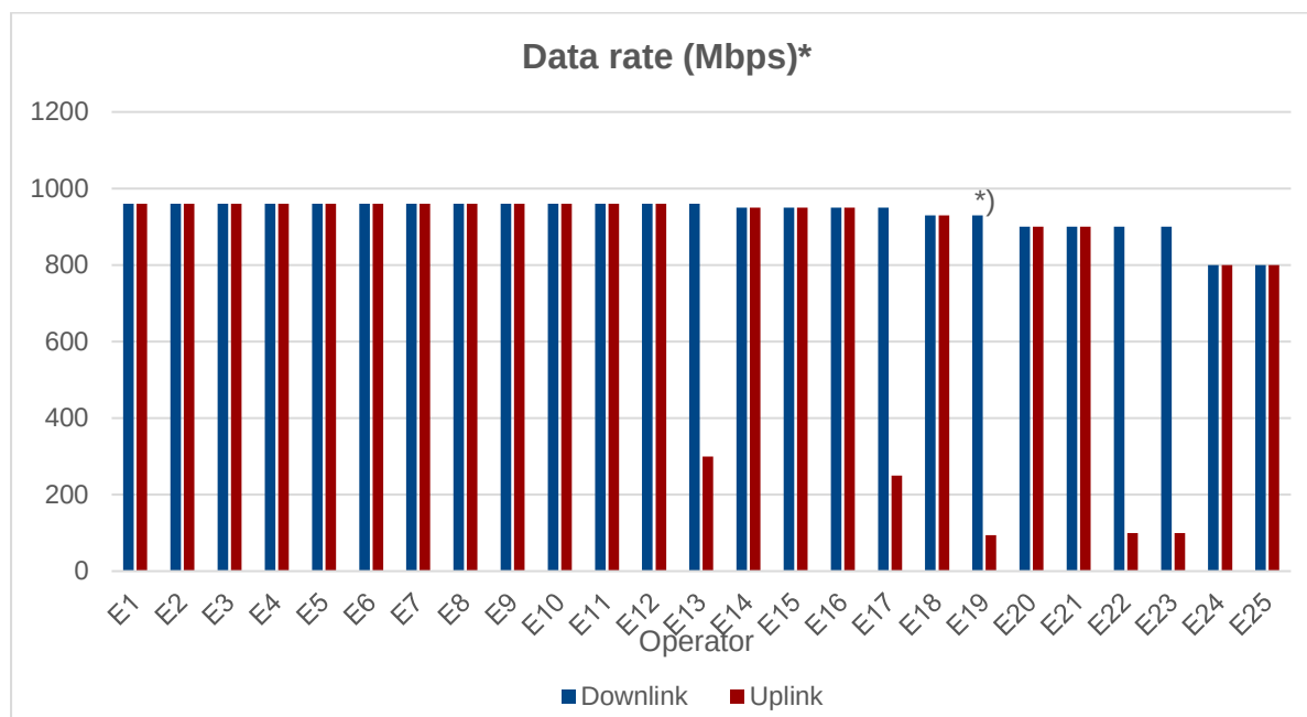
Figure 12: Typically achievable data rates during peak-time in fixed networks with fibre to the multi-dwelling building and Gigabit Ethernet on the in-building twisted pair cable of category 5 or higher
