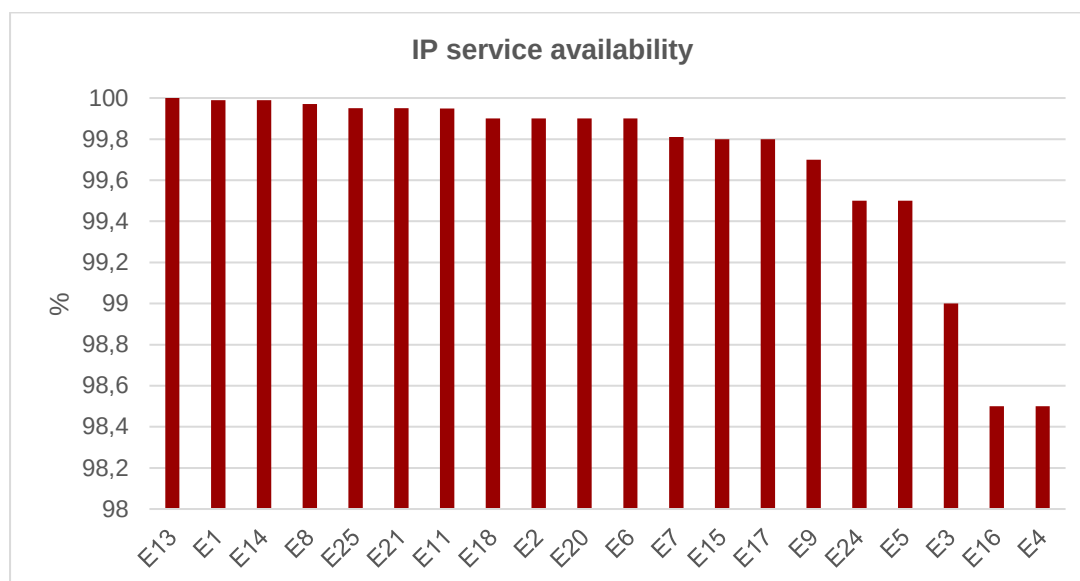
Figure 15: Typically achievable IP service availability in fixed networks with fibre to the multi-dwelling building and Gigabit Ethernet on the in-building twisted pair cable of category 5 or higher
