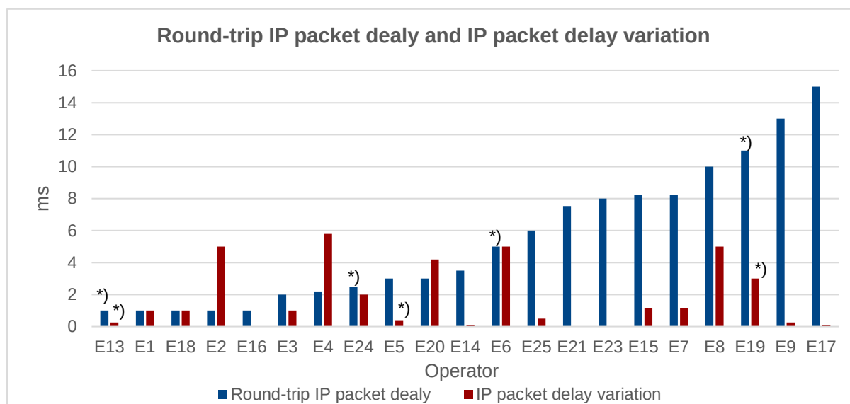
Figure 14: Typically achievable round-trip IP packet delay and IP packet delay variation in fixed networks with fibre to the multi-dwelling building and Gigabit Ethernet on the in-building twisted pair cable of category 5 or higher
