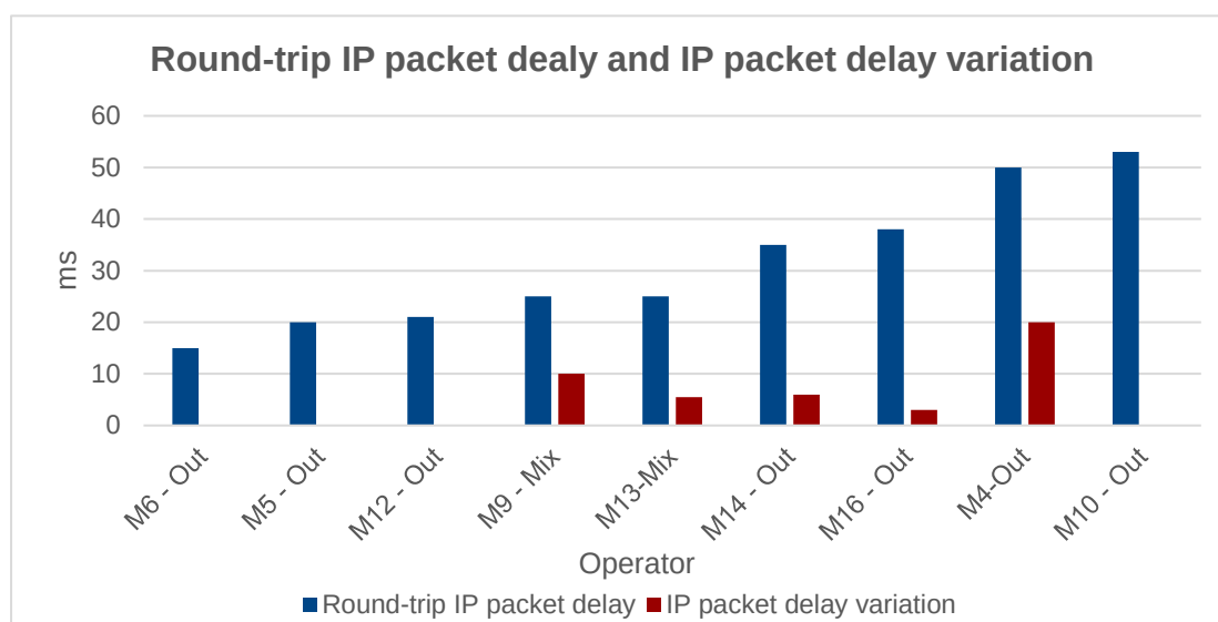
Figure 10: Average value of the achievable round-trip IP packet delay and IP packet delay variation during peak-time in a mobile network with fibre roll-out up to the base station and the best LTE Advanced technology used in this network
