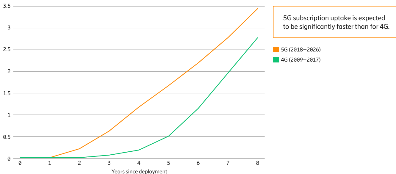
Figure 2: Comparison of 5G and 4G subscriptions uptake in the first years of deployment (billion)
