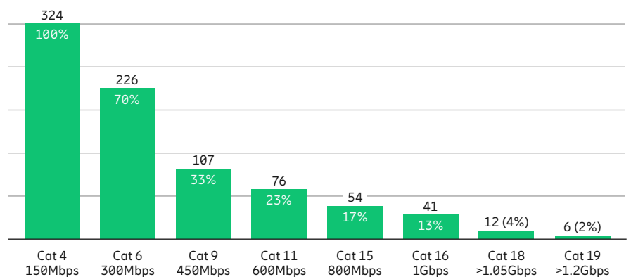
Figure 18: Percentage and number of LTE-Advanced networks supporting various categories of devices
