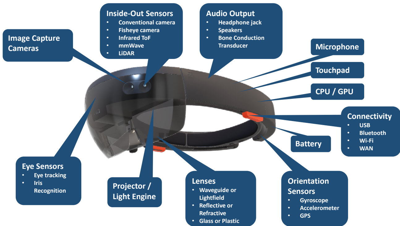
Figure 2: AR Glasses Components (Source: Strategy Analytics)
