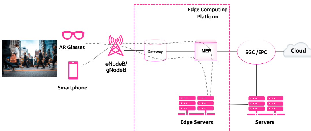
Figure 16: Significant parts of Augmented Computing can be done at the Edge (Source: Strategy Analytics Service Provider Group)
