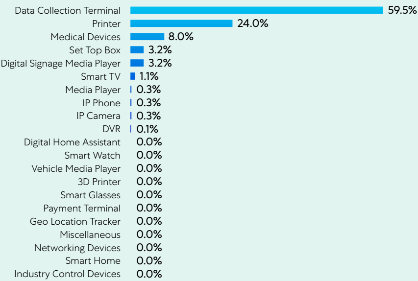
Base: 575,091,158 IoT device transactions Figure 2: IoT device transactions
