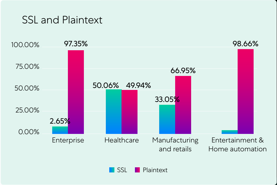
Figure 4: Percentage of encrypted communications by device type
