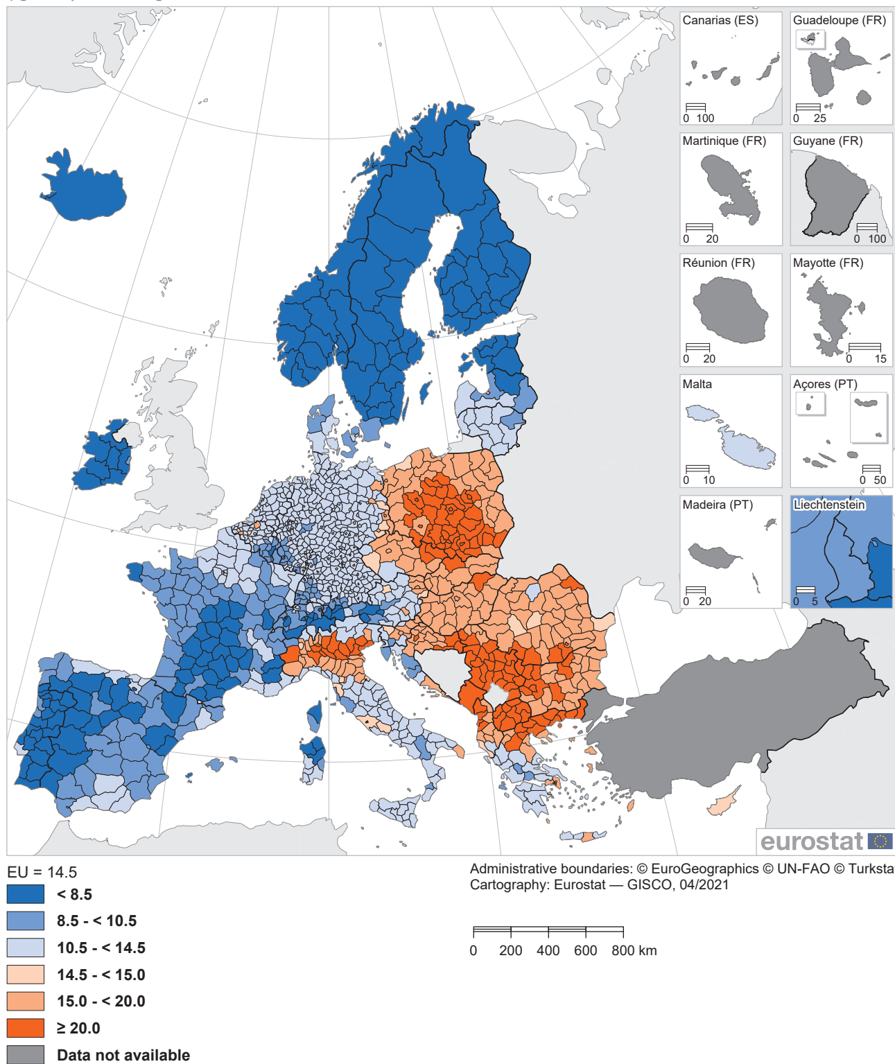
Map 12.3: Exposure to air pollution by fine particulate matter (PM 2.5 ), 2018 (µg/m 3 , by NUTS 3 regions)
