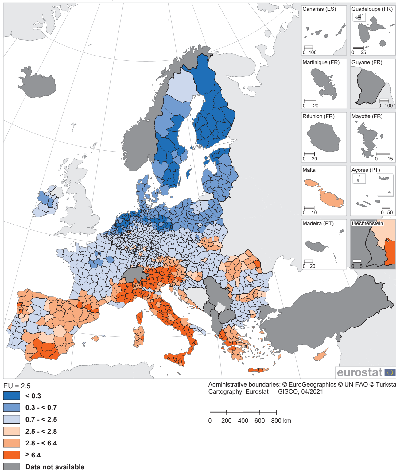
Map 12.5: Soil loss by water erosion, 2016 (tonnes per hectare, by NUTS 3 regions)
