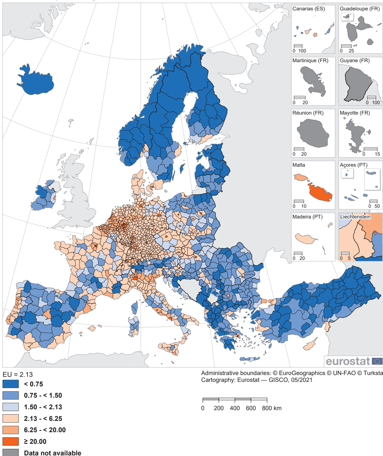
Map 12.4: Sealed soil surfaces with impervious materials, 2018 (% of total area, by NUTS 3 regions)
