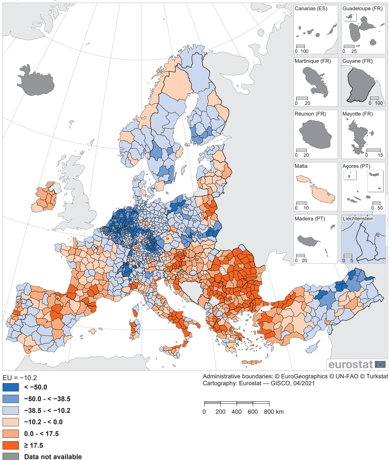
Map 12.6: Overall change in soil moisture, 2000-2019 (%, by NUTS 3 regions)
