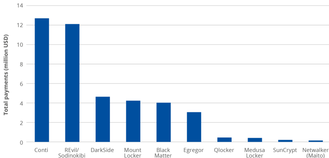
Figure 6: Ransomware data, grouped by family, in 2021. (Source: https://ransomwhe.re/ )
