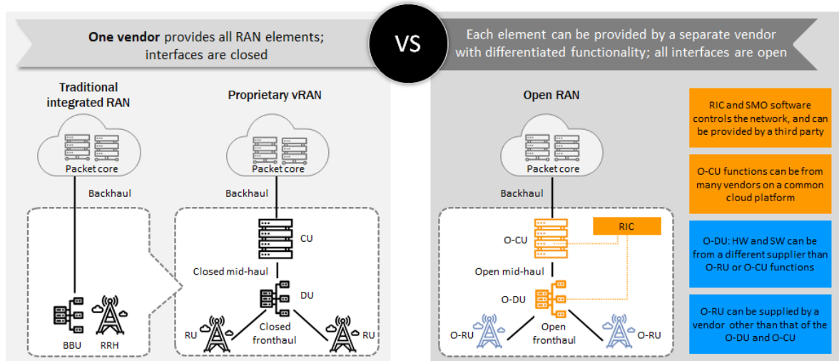
Figure 1. Disaggregation and open interfaces in Open RAN vs Traditional RAN
