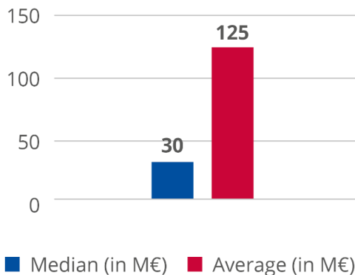
Figure 9: IT spending
