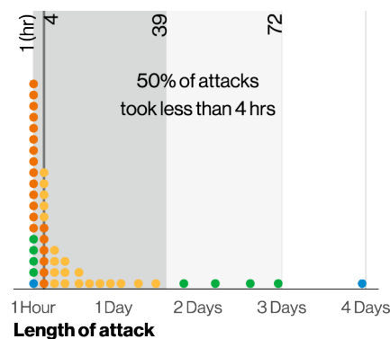
Figure 65. DDoS attack duration (n=15,059 log scale)
