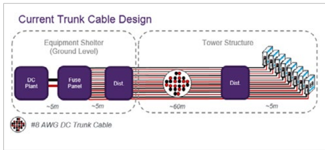
Figure 13: Current approach to DC power distribution network based on trunk cables. The figure shows a single sector with 8 RU's, where each RU is individually fed from the DC power source in the equipment shelter at the base of the tower
