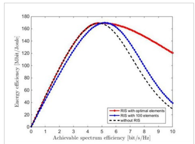
Figure 16: Energy Efficiency of 5G-NR RIS assisted v 5G-NR Baseline system
