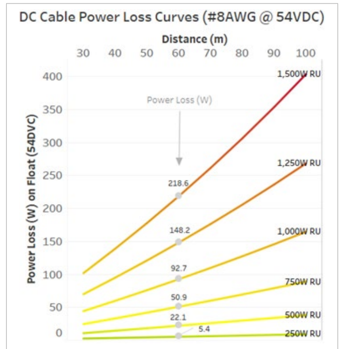
Figure 11: DC power losses calculated using two-way distances with typical #8 AWG DC trunk cables. Note the exponential relationship between the RU power consumption and the DC power losses due to the I 2 R law (i.e. for the same conductor size, the doubling of the DC current results in the quadrupling of the DC power losses)
