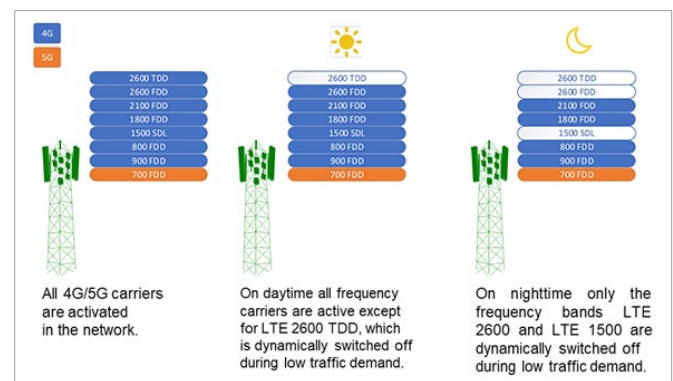
Figure 3: Example of carrier shutdown in 4G network
