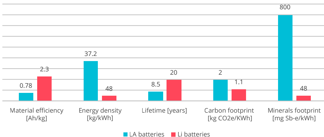
Figure 3.2: Material efficiency and environmental impact in comparison of LA and Li batteries
