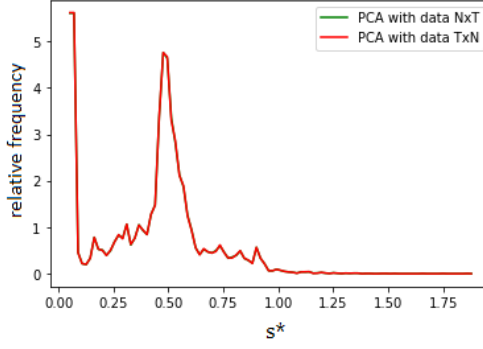
Figure 10: Comparison between the anomaly scores histograms obtained by running PCA on data in the formats N \times T and T \times N .
