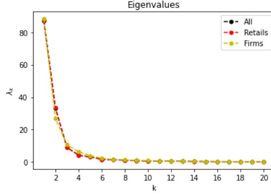
Figure 19: IMA. Eigenvalues obtained by performing PCA using the whole dataset ( All ), the dataset made up of households ( Retails ) and the dataset made up of firms ( Firms ).
