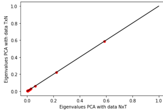
Figure 9: Comparison between the eigenvalues obtained by running PCA on data in the formats N \times T and T \times N . The dark line is the bisector.
